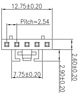
HOUSING (DETAIL-B)
